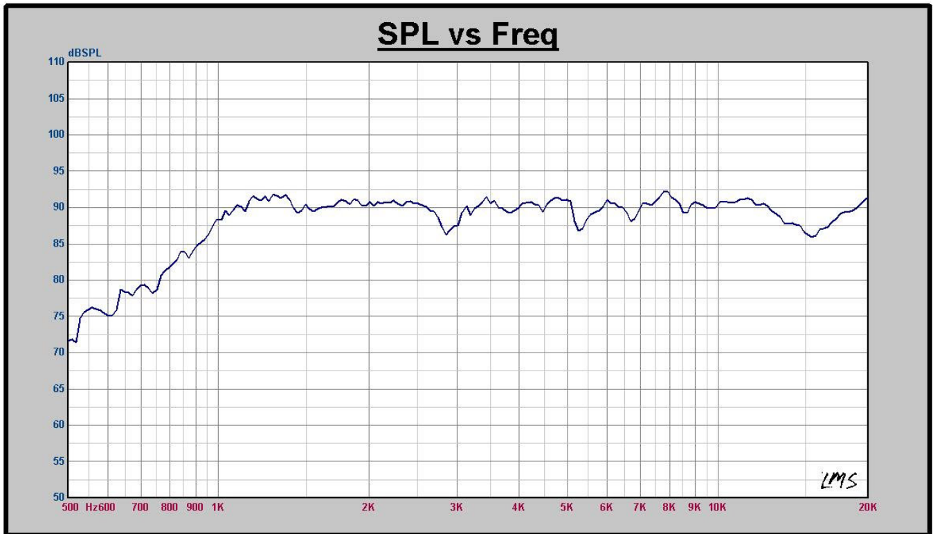
FIG. 1: FREQUENCY VS.SPL
