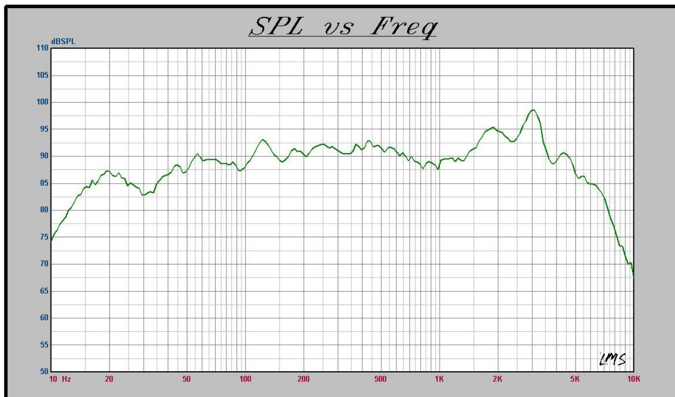
FIG. 1: FREQUENCY VS.SPL
