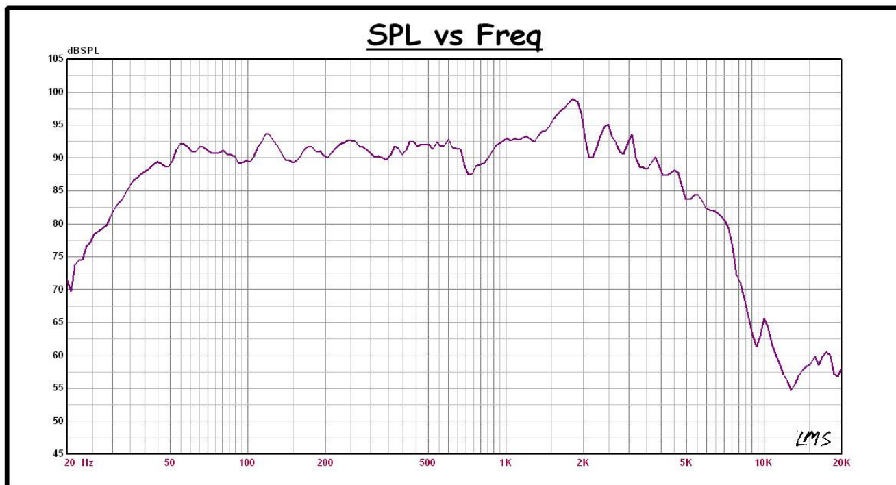
FIG. 1: FREQUENCY VS.SPL
